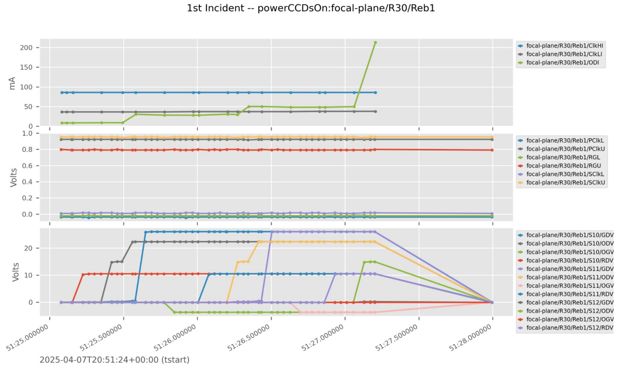
FIGURE 3: Trending of the first power-on attempt (Marshall, 2025). Top: the REB parent currents, with ODI (green) leaving its baseline as the bias sequence proceeds and reaching 213 mA. Middle: the clock rails. Bottom: the CCD bias voltages; the last trace to rise, to \approx 15 V, is the OD of S12, and all biases return to zero at 51:28 when the protection has fired and powerCCDsOff runs.
